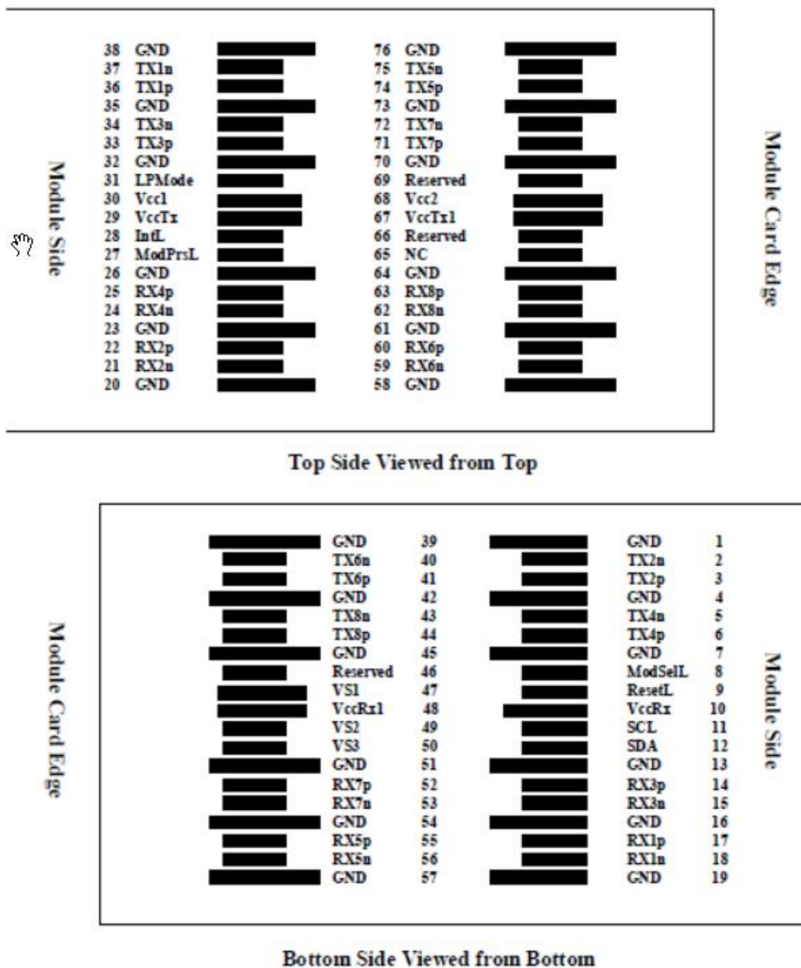
Figure1 QSFP-DD MSA-compliant 76-pin connector
