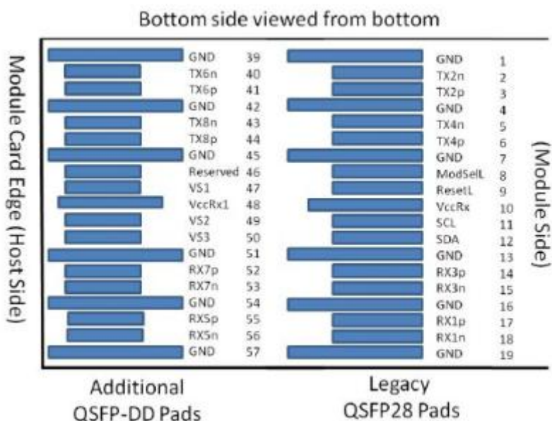
Figure1 QSFP-DD MSA-compliant 76-pin connector
