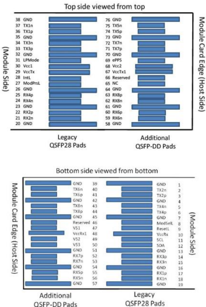
Figure1 QSFP-DD MSA-compliant 76-pin connector
