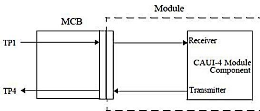
Figure 1: Module CAUI-4 compliance test point
